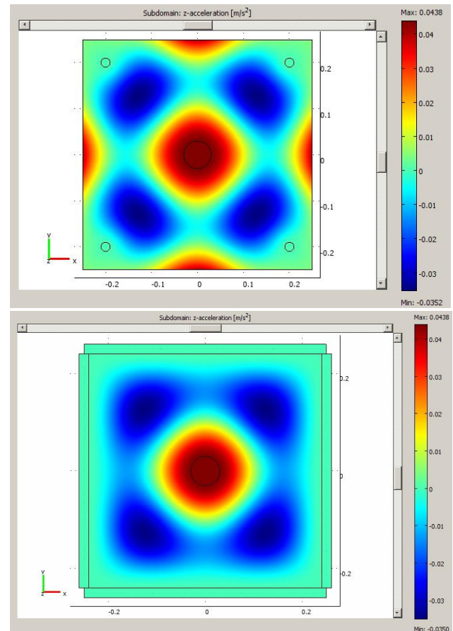
Figure 6: Numerical simulation of the glass plate at 1000 Hz having the transducer in the center and with screw fixings at the corners (top) and using a frame (bottom). Small circles in the top image show simulated wall-fixing points where displacement of the plate is zero.
